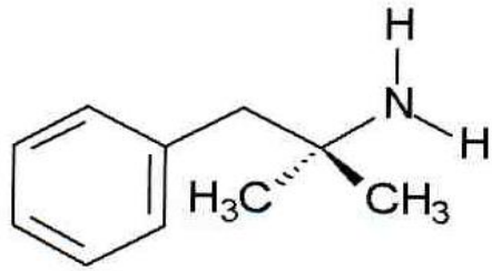
Phentermine
