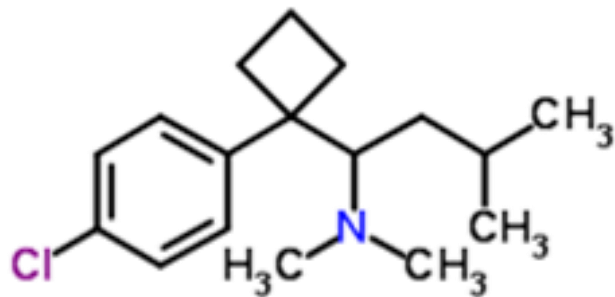
Sibutramine
